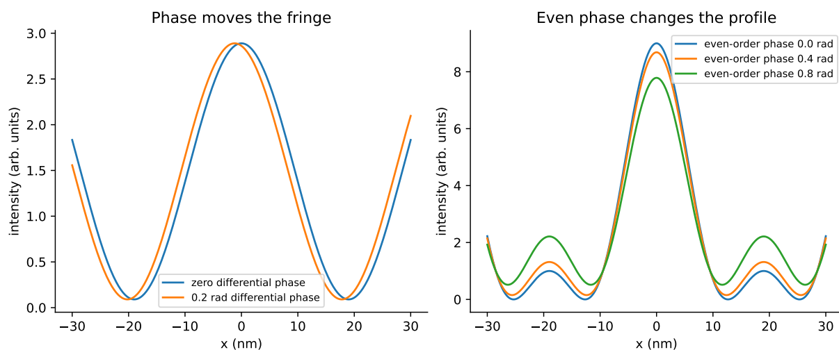
Figure 8.2: Exact teaching examples. A differential phase between two orders shifts fringes. A common phase on symmetric side orders changes an even intensity profile. A real contact combines many such interference terms and an incoherent source average.
