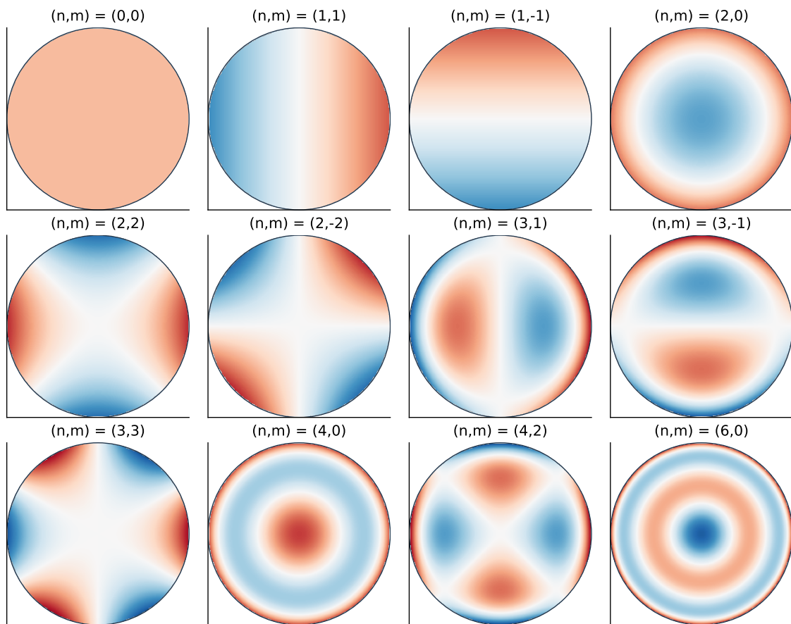
Figure 7.1: Original atlas of selected real, RMS-normalized modes. Red and blue indicate opposite OPD signs; the same colour scale is used throughout. The labels are (n, m) , not the paper's single-index coefficient numbers.
