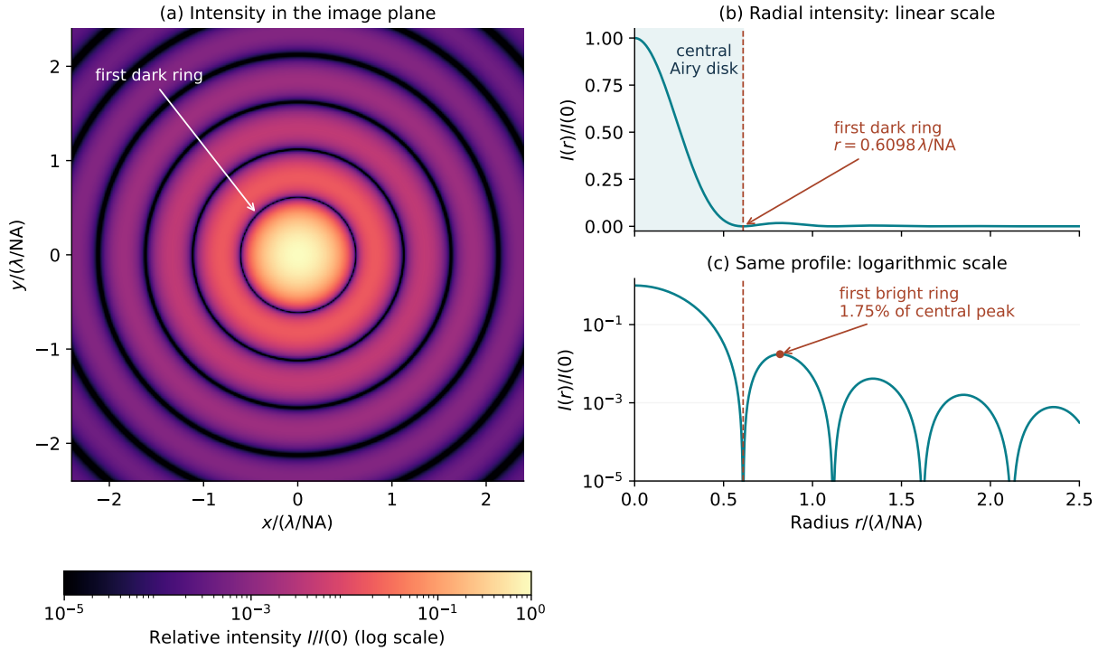
Figure 4.1: Airy intensity pattern for a uniformly illuminated, unobscured circular pupil with no aberration. Coordinates are measured in units of \lambda/\text{NA} , and intensity is normalized to its on-axis value. (a) The image-plane pattern uses a logarithmic colour scale to reveal the faint rings; colour does not represent wavelength. (b) The radial intensity on a linear scale shows the dominant central spot. The dashed line marks the first dark ring at r = 0.6098\lambda/\text{NA} . (c) The same radial profile on a logarithmic scale reveals the outer rings. The first bright ring reaches only about 1.75 percent of the central peak. The logarithmic displays stop at I/I(0) = 10^{-5} ; the ideal dark-ring minima are zero.
